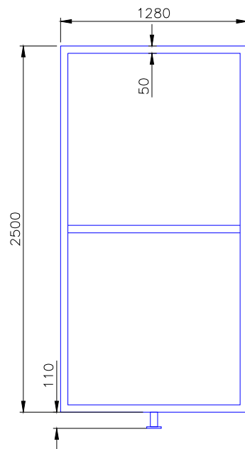
4 of 50 x 50 x 3 EA 50 x 5 T Flat Pt No TP008
