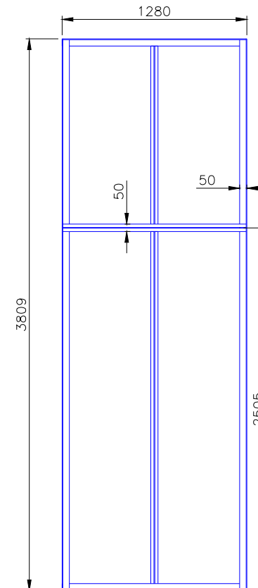
2 of 50 x 50 x 5 EA 50 x 50 x 6 T Section Pt No TP006
